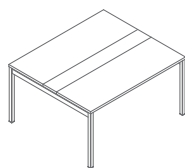
SY44 1400 / 1210 / 740 60.15 kg
