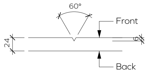
V-cut Detail
