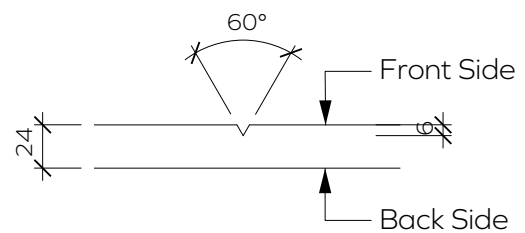
V-cut Detail
