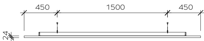
Front
