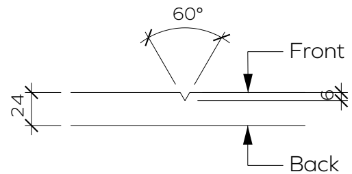
V-cut Detail
