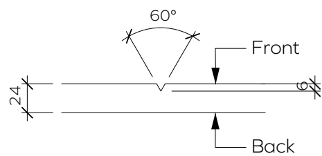
V-cut Detail
