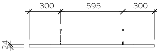
Front
