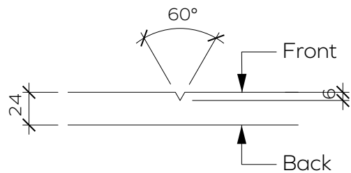
V-cut Detail
