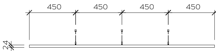
Front
