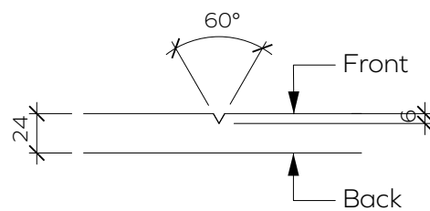
V-cut Detail
